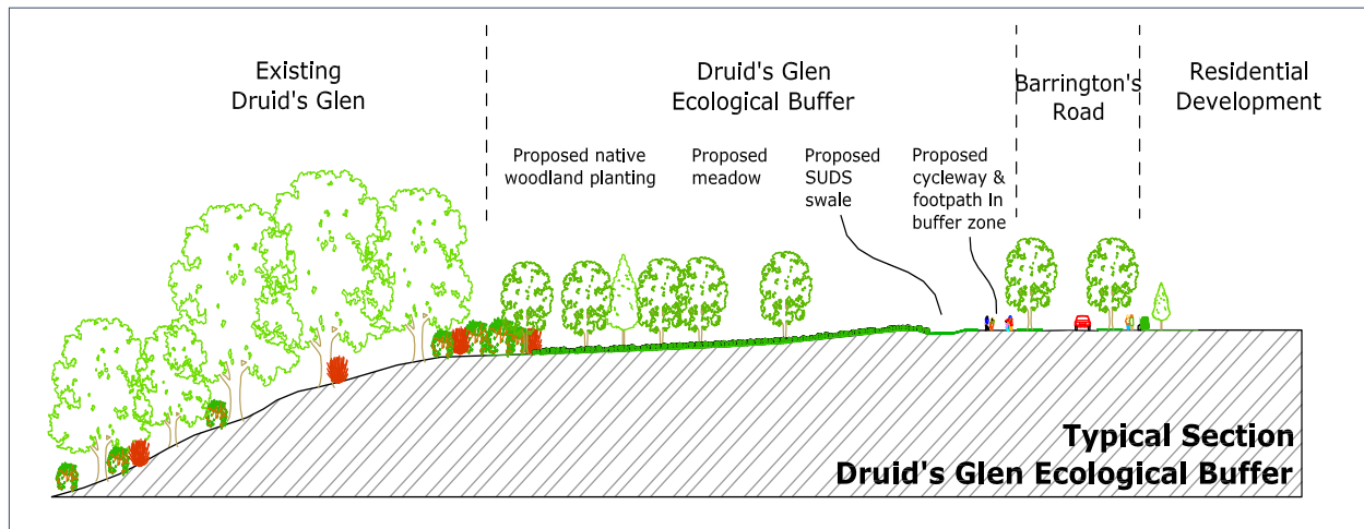
Figure 5.2: Typical Section Through Druid's Glen Ecological Buffer
