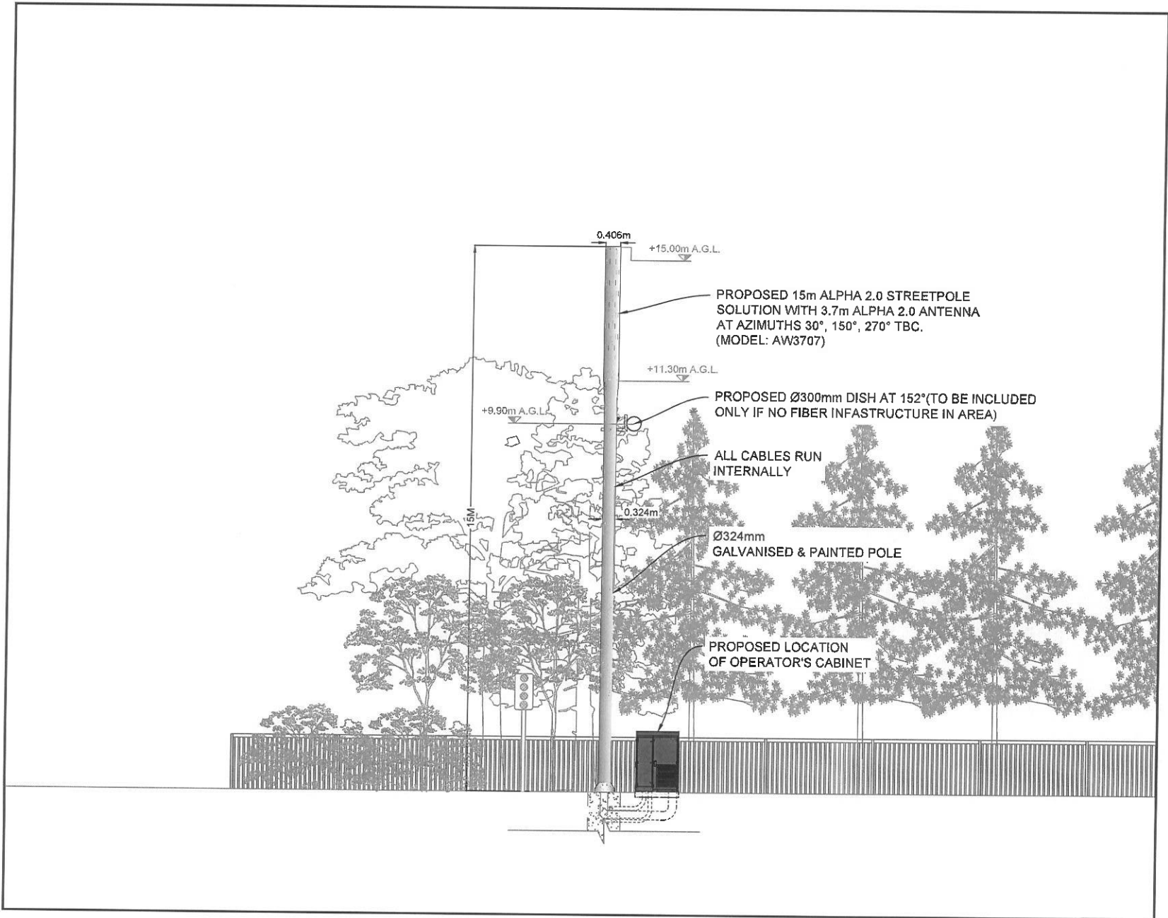
ELEVATION SCALE 1:100
