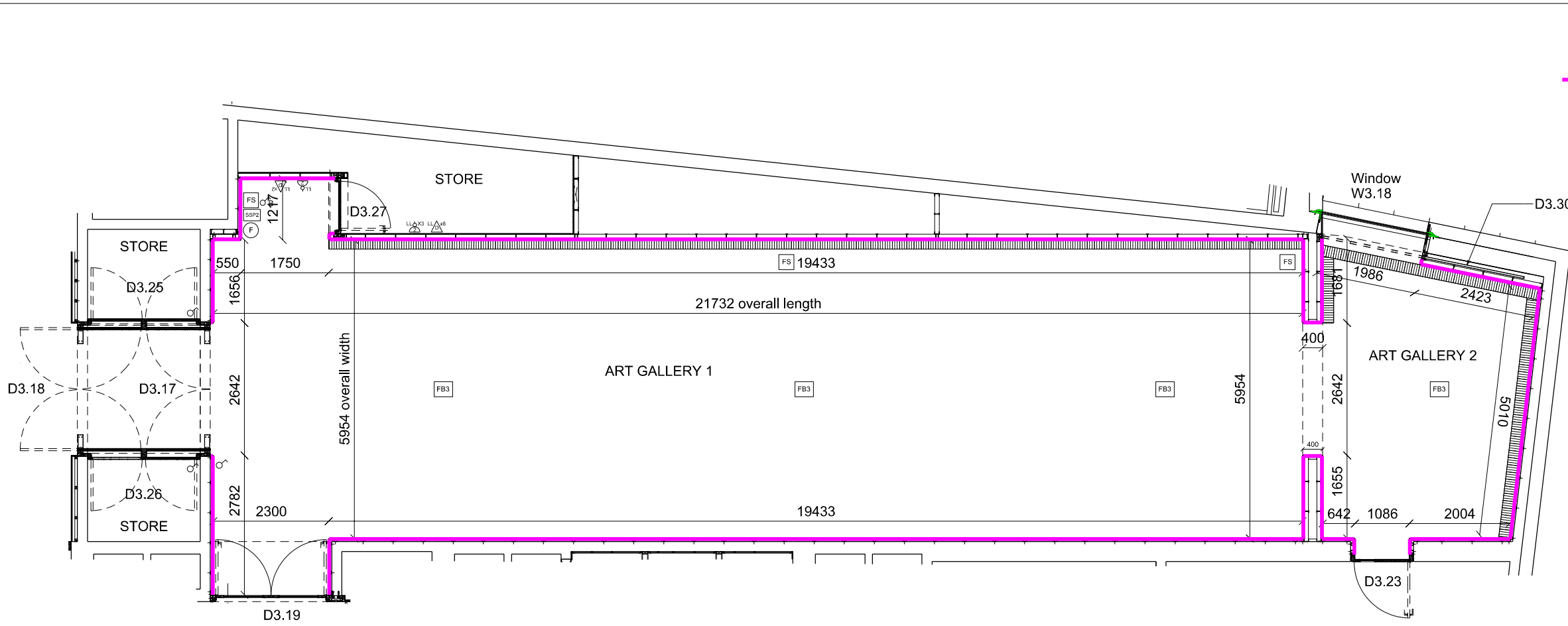
FLOOR PLAN
