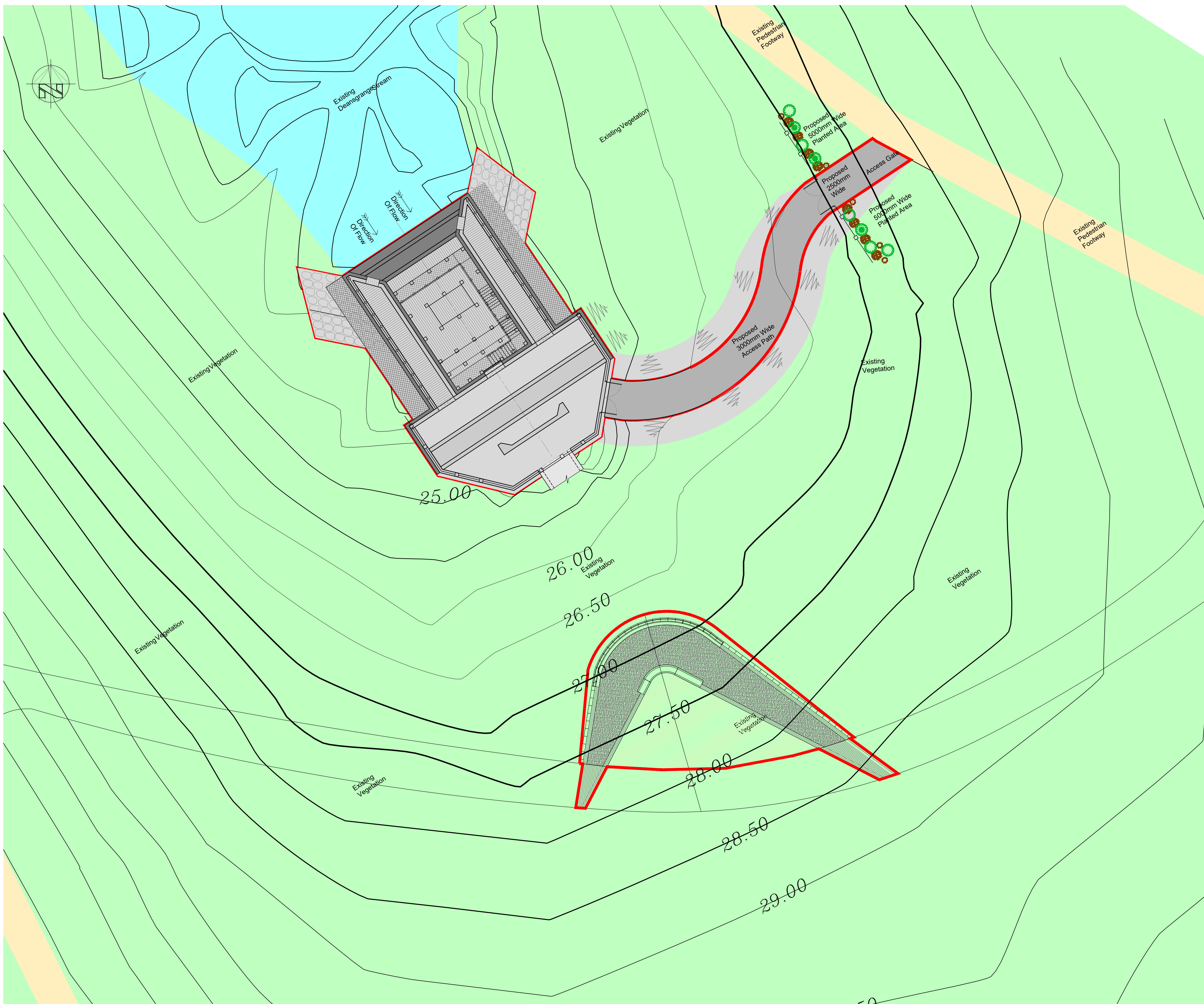
FLOW CONTROL STRUCTURE & VIEWING PLATFORM LAYOUT PLAN SCALE: 1:150
