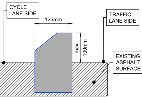
DETAIL A - INDICATIVE SEGREGATION KERB DETAIL
