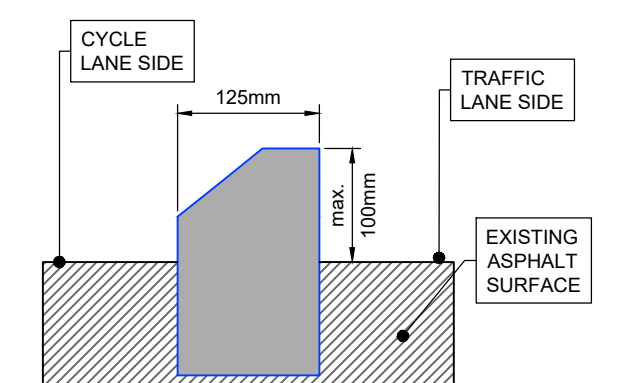
DETAIL A - INDICATIVE SEGREGATION KERB DETAIL
