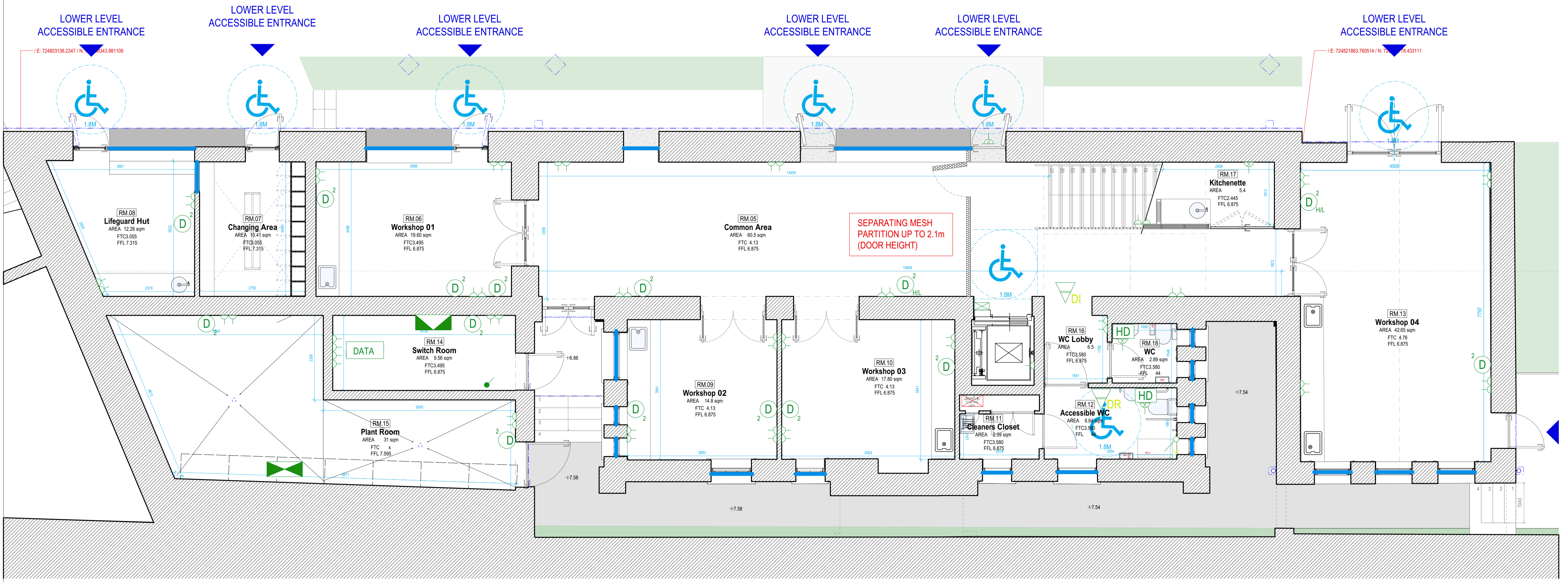
4 Lower Level Access Plan 200 Scale: 1:50 @ A1
